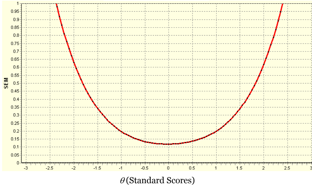
Figure 1. IRT Functions for a Peaked Conventional Test
