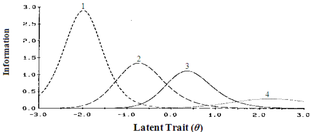
Figure 5. IFFs for Four Dichotomously Scored Items
