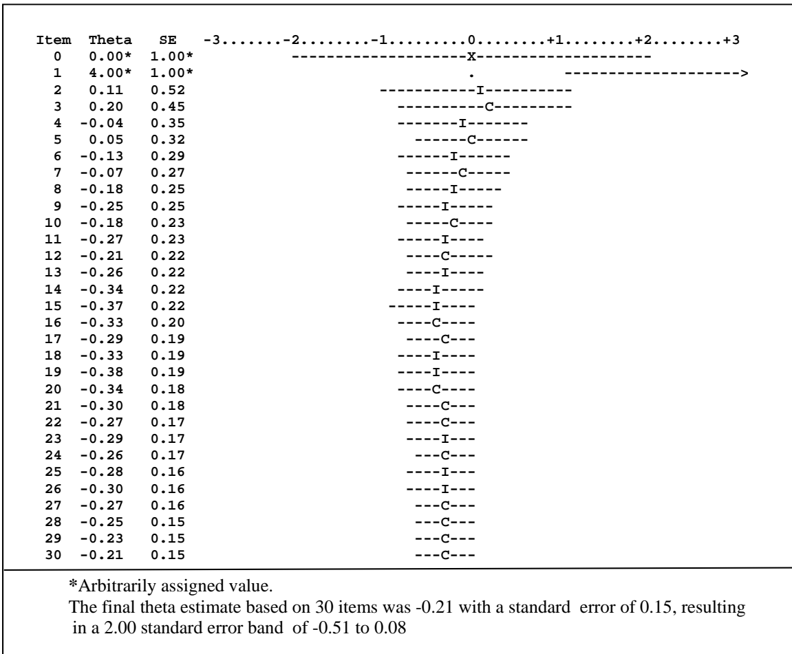
Figure 8. A Sample Report on an IRT-Based Adaptive Test for a Different Examinee
