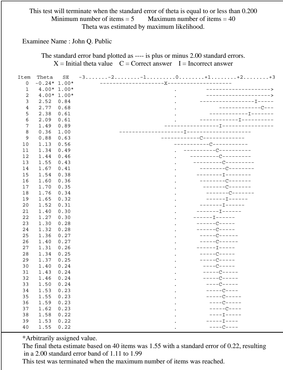
Figure 7. A Sample Report on an IRT-Based Adaptive Test
